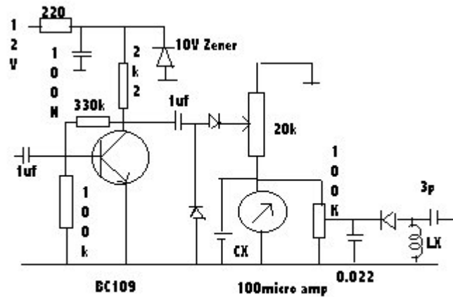
Relative pwr/S meter - G4KIH GQRP 3806
