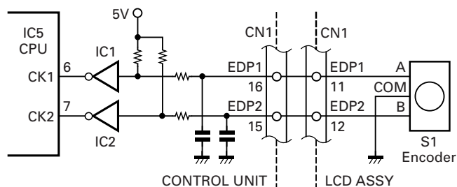
Fig. 12 Encoder circuit
