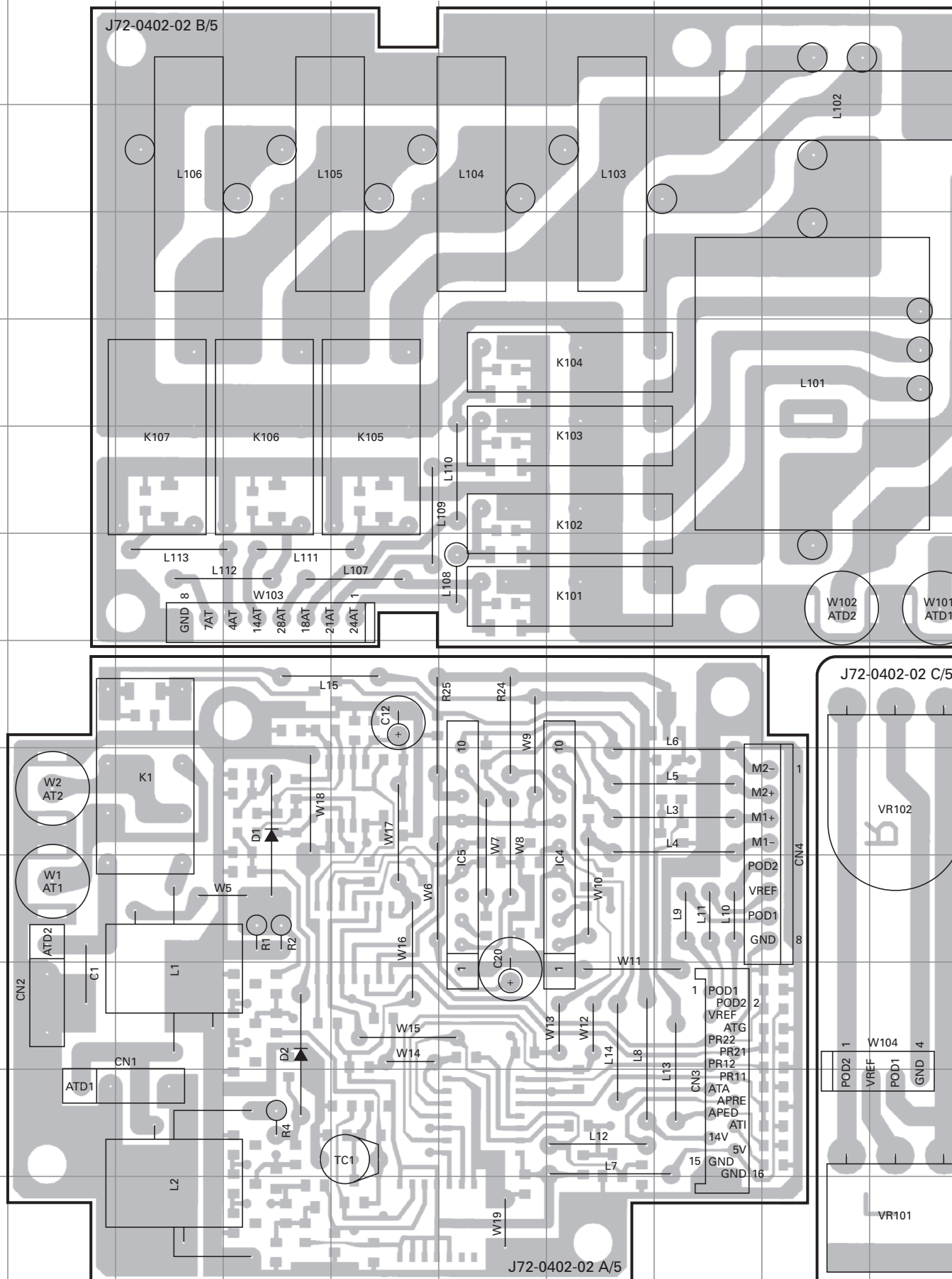
AT UNIT (X53-3630-20) Component side view (J72-0402-02)
