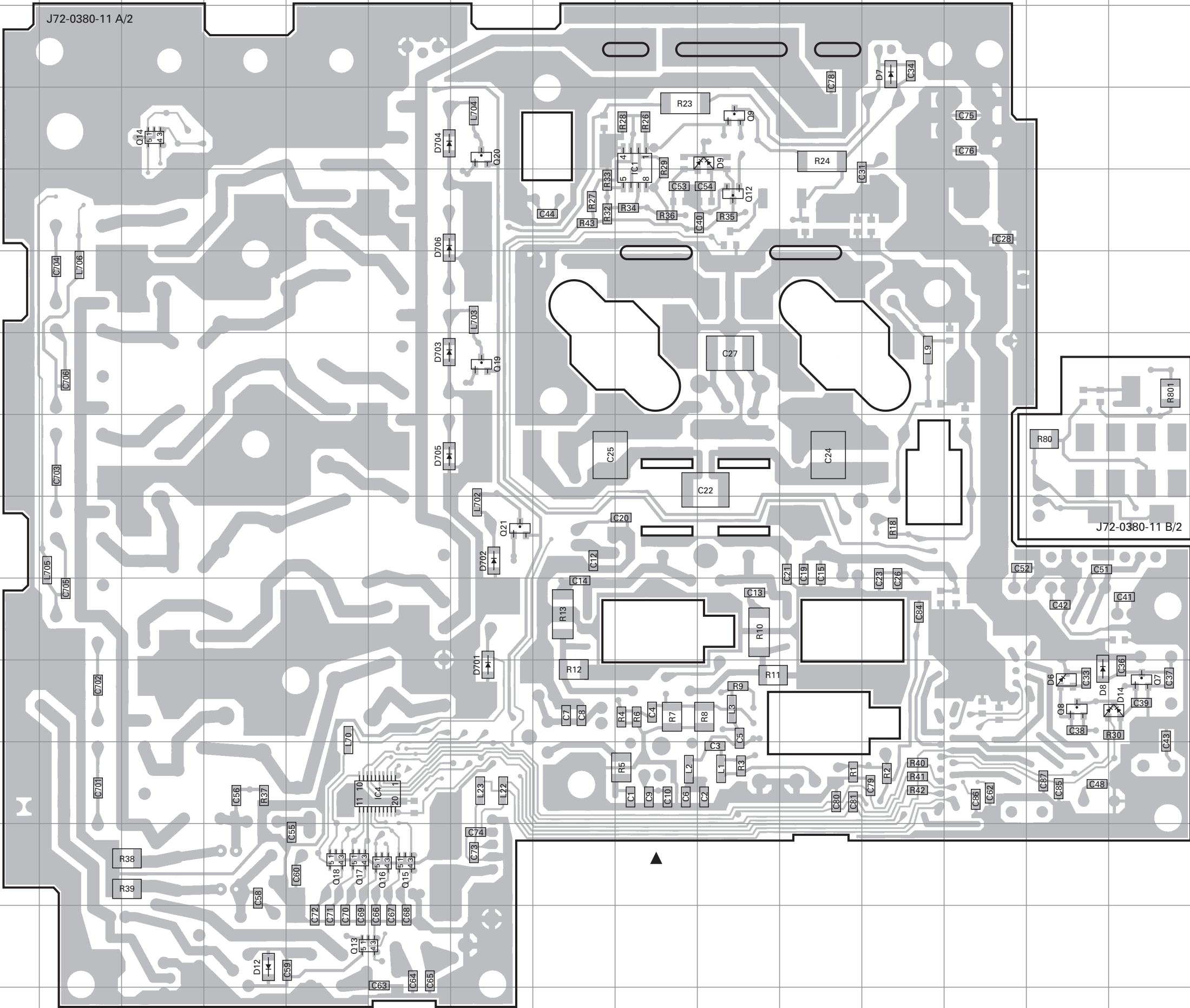
FINAL UNIT (X45-3520-21) Foil side view (J72-0380-11)
