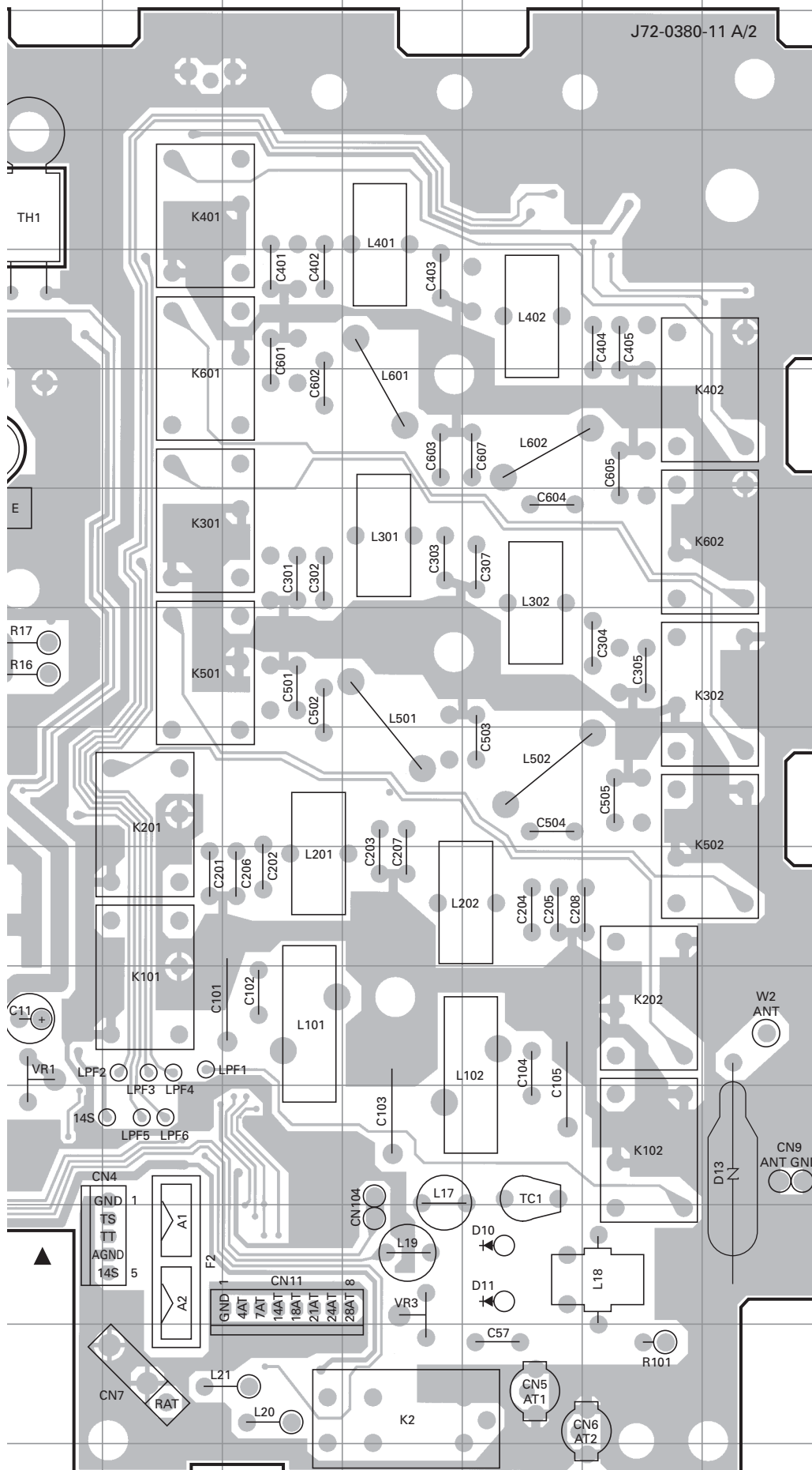
FINAL UNIT (X45-3520-21) Component side view (J72-0380-11)
