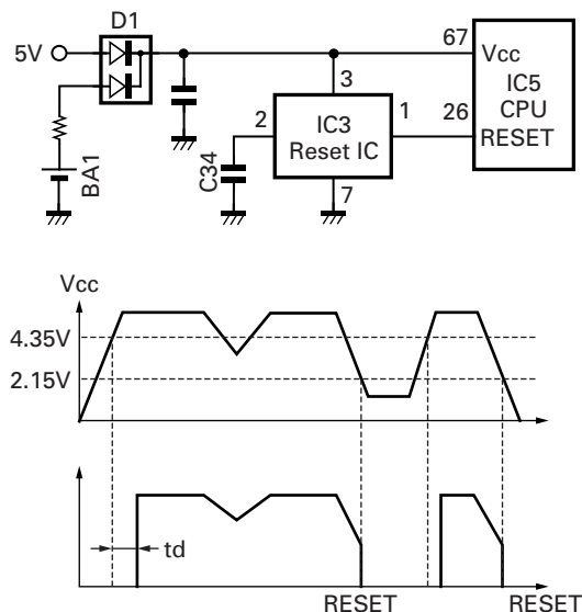
Fig. 9 Reset circuit
