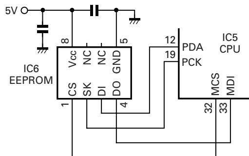
Fig. 11 EEPROM circuit
